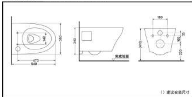
CW582EB Toilet with Concealed Flush Tank
