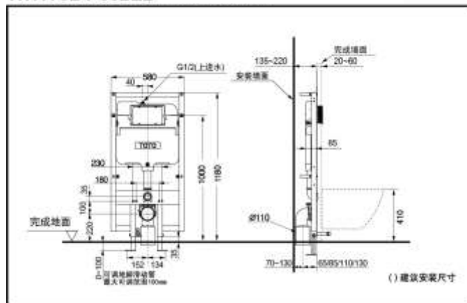
WH173BT-582EB Concealed Flush Tanks
