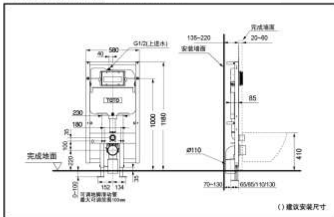
WH173B-582EB Concealed Flush Tanks
