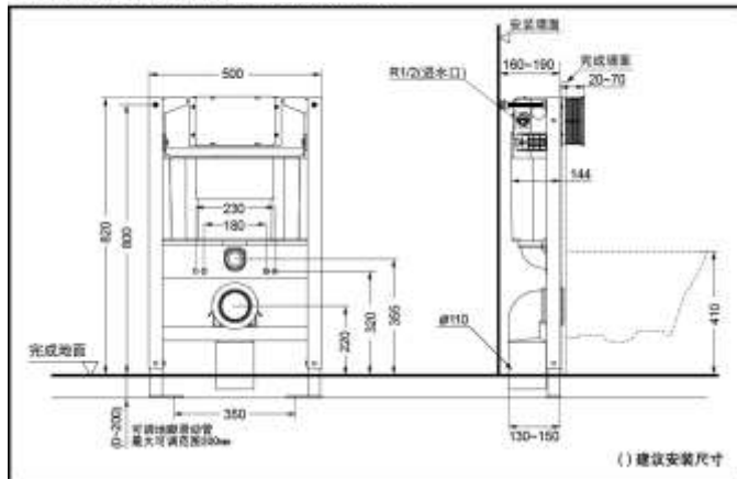
WH143B-582EB Concealed Flush Tanks
