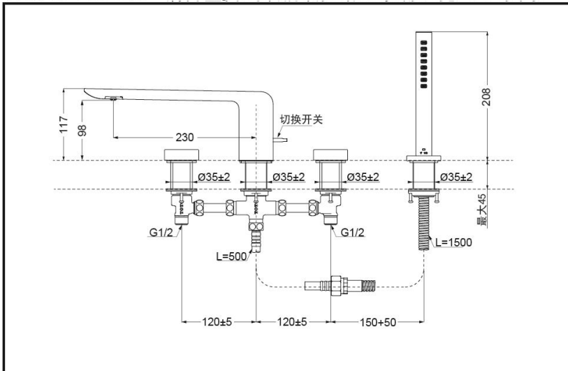
TBP02202B1 Deck-Mounted Bathtub Double Lever Mixer(W/ Hand Shower)
