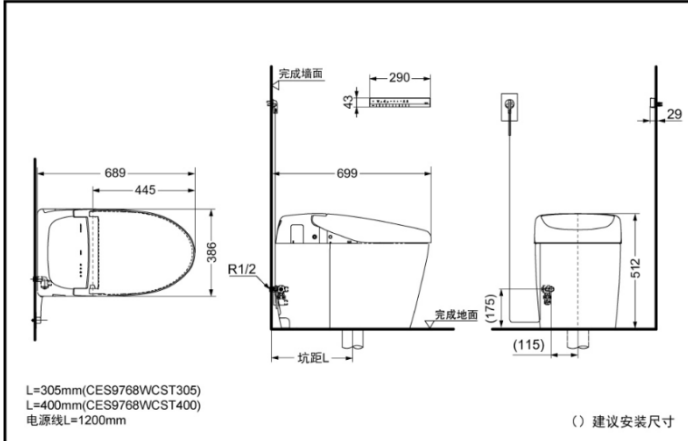
CES9768WCST305/CES9768WCST400 NEOREST One-piece Toilet/Bidet
