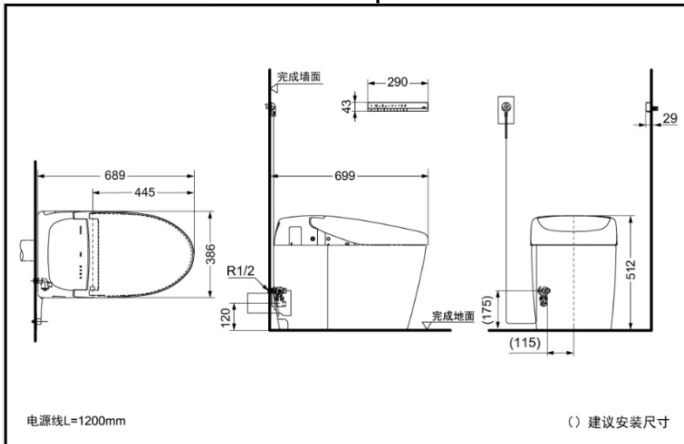
CES9768PWCS NEOREST One-piece Toilet/Bidet
