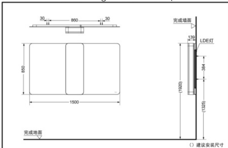
LMFW1501DW Dressing Mirror Cabinet (RENESE series)
