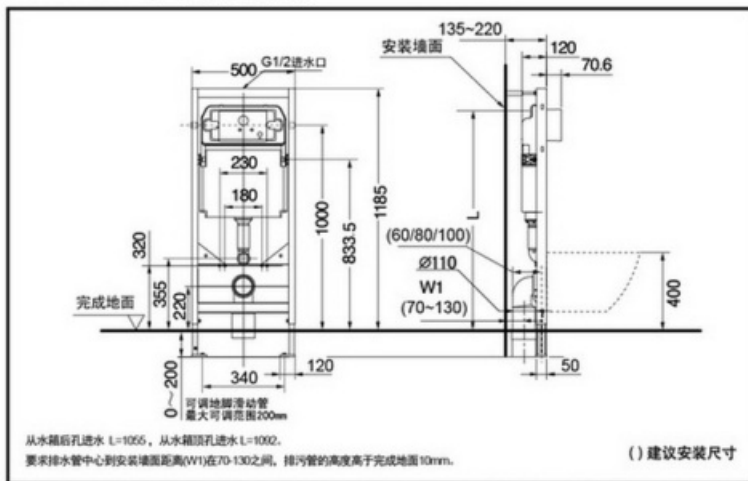
WH023R Concealed Flush Tank
