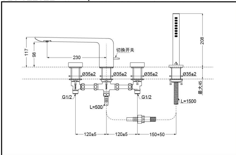
TBP02202B Deck-Mounted Bathtub Double Lever Mixer(W/ Hand Shower)
