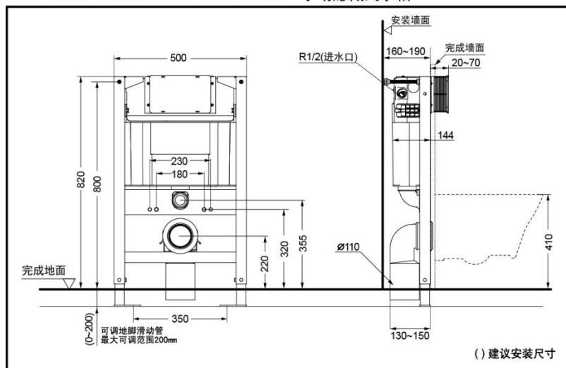
WH142B-162B/WH142B-762B 手动隐藏式水箱
