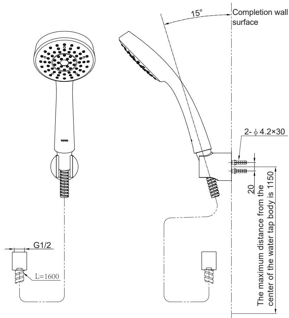
TBW01017* series "L Shower" 1mode Hand Shower Set (Standard Type)
